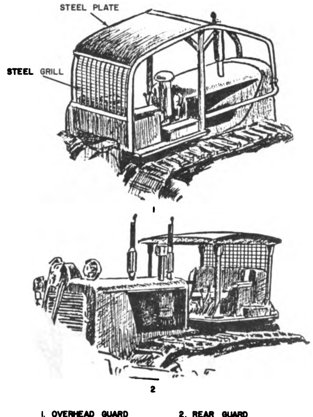
1. OVERHEAD GUARD 2. REAR GUARD Figure 7-1. Guards to protect the tractor operator.
